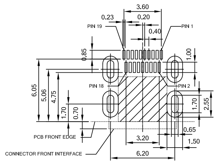
RECOMMENDED PCB LAYOUT <TOP VIEW> TOLERANCE : ± 0.05mm
