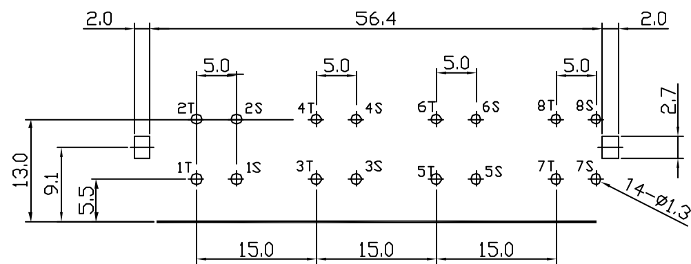
PCB LAYOUT
